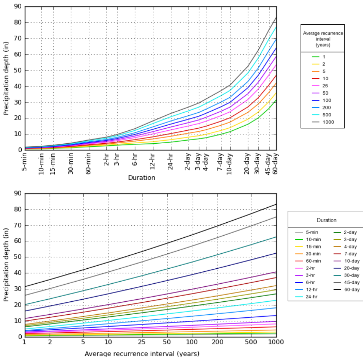
Figure 5.3.3. Sample depth-duration-frequency curves built from the PDS data with duration on the x-axis (top figure) and average recurrence interval on the x-axis (bottom figure).
