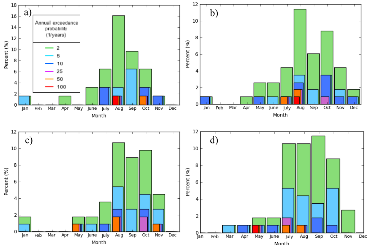
Figure A.9.1. Example of seasonal exceedance graphs for the: a) 60-minute, b) 24-hour, c) 2-day, and d) 10-day durations.
