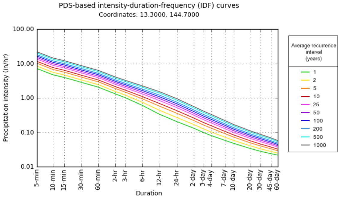
Figure 5.3.4. Sample intensity-duration-frequency (IDF) graph with duration on the x-axis.
