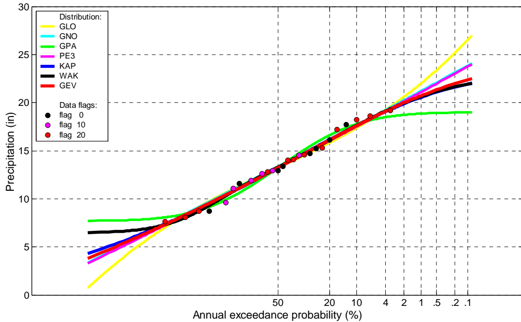
Figure 4.5.2. Probability plots for selected distributions for 7-day AMS at station 91-4594 (Tutuila, AS). Data quality flags were assigned to all annual maxima during the extraction process to assist in data quality control described in Section 4.3.2.
