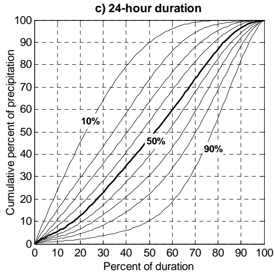
Figure 5.3.7. Sample temporal distribution curves for 24-hour all cases.
