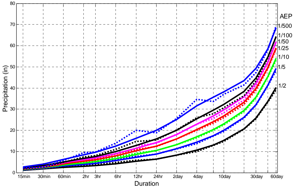
Figure 4.5.3. Precipitation frequency estimates for a range of durations for selected AEPs for station 91-4594 (Tutuila, AS). Dotted lines represent original estimates; full lines represent estimates obtained after L-moments were smoothed across durations.
