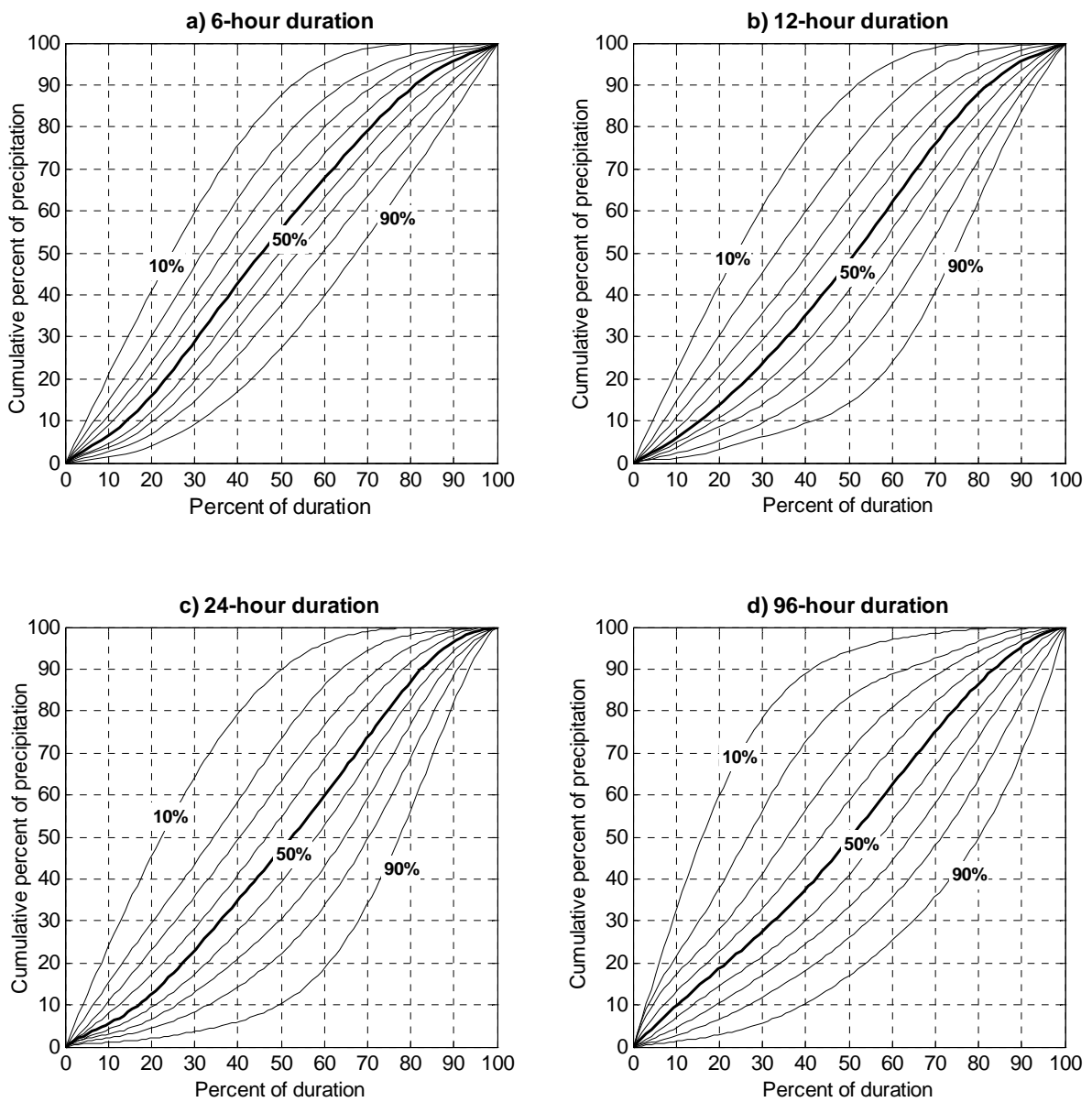
Figure A.8.1. Temporal distribution curves for all cases for: a) 6-hour, b) 12-hour, c) 24-hour, and d) 96-hour durations.
